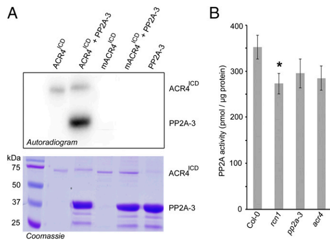
Fig. 3. PP2A-3 is phosphorylated by ACR4 kinase. (A) Autoradiogram for coincubated E. coli -expressed PP2A-3 and ACR4 kinase (ACR4 ICD ) or mutant inactive kinase mACR4 ICD as indicated (Upper). The lanes in A are, from left to right, molecular weight standards, 1 μg of autophosphorylated ACR4 ICD , 1 μg of autophosphorylated ACR4 ICD incubated with 10 μg PP2A-3, 1 μg of mutant inactive kinase mACR4 ICD incubated with 10 μg PP2A-3, and 10 μg PP2A-3. Corresponding Coomassie blue-stained gel (Lower) was used as loading control. (B) Bar diagram for PP2A activity detected in whole 12-d-old seedling protein extracts as average of three biological repeats (with three technical repeats each) ± SE. Statistical significance (Student's t test) compared with Col-0 is indicated: * P value < 0.05.
